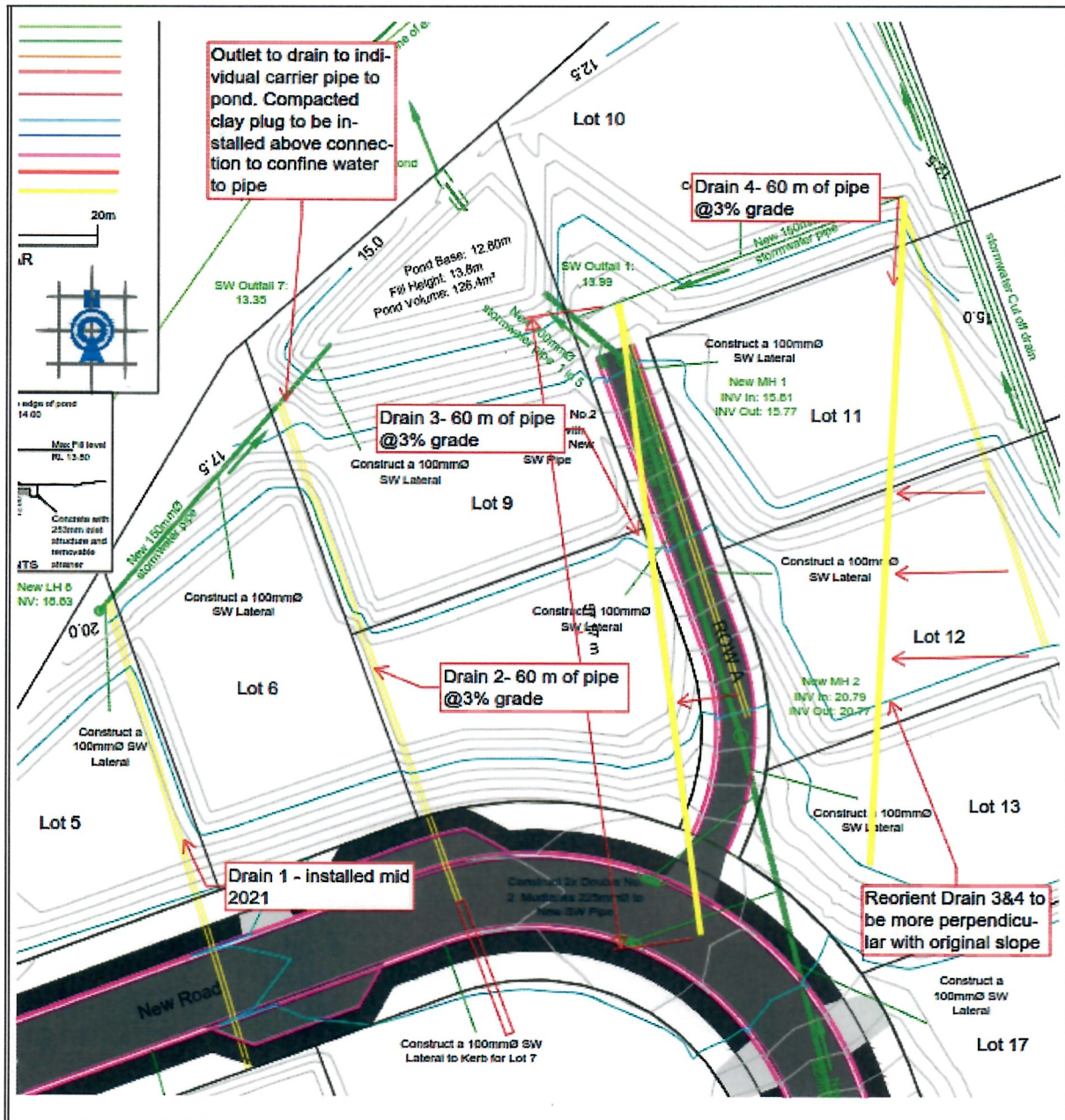
Figure 1: Deep horizontal drain locations. Upslope location and depths of pipe to be confirmed by contractor.
